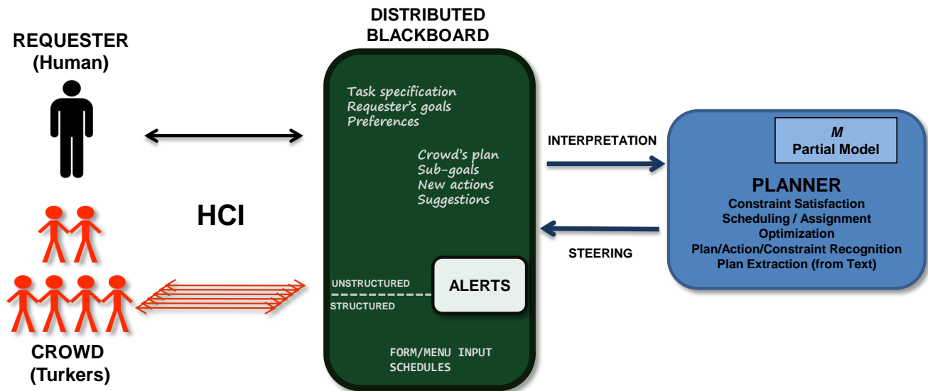
Figure 1: An architecture for planning in crowdsourced planning systems.
